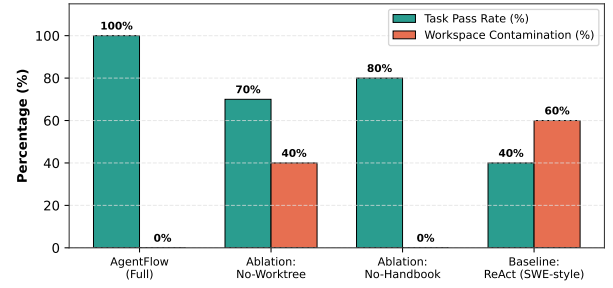
Figure 5: Comparative Benchmark & Ablation across 10 Micro-Scenarioic
