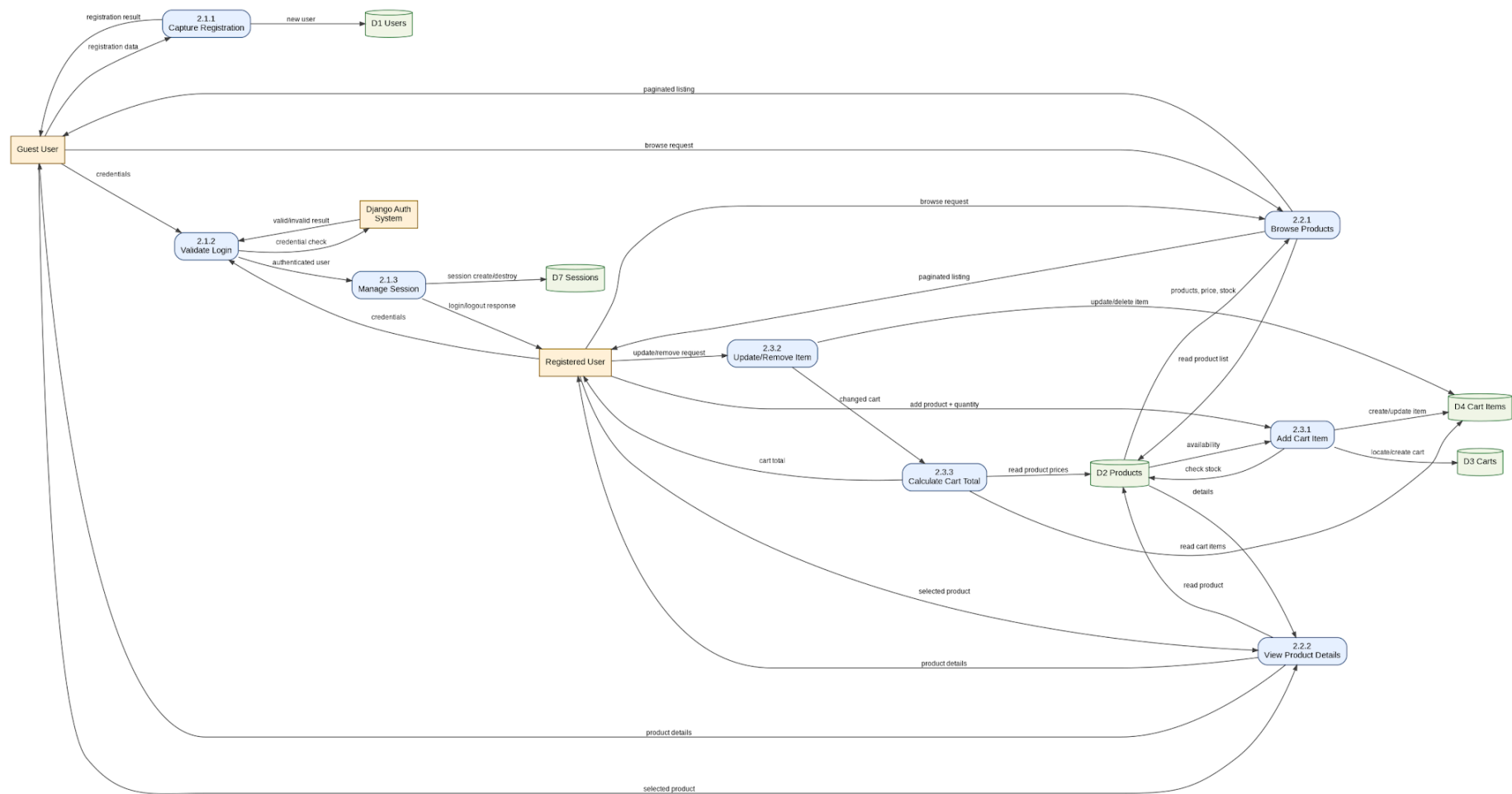
Figure 1: Level-2 DFD - Authentication, Product Browsing, and Cart Management
