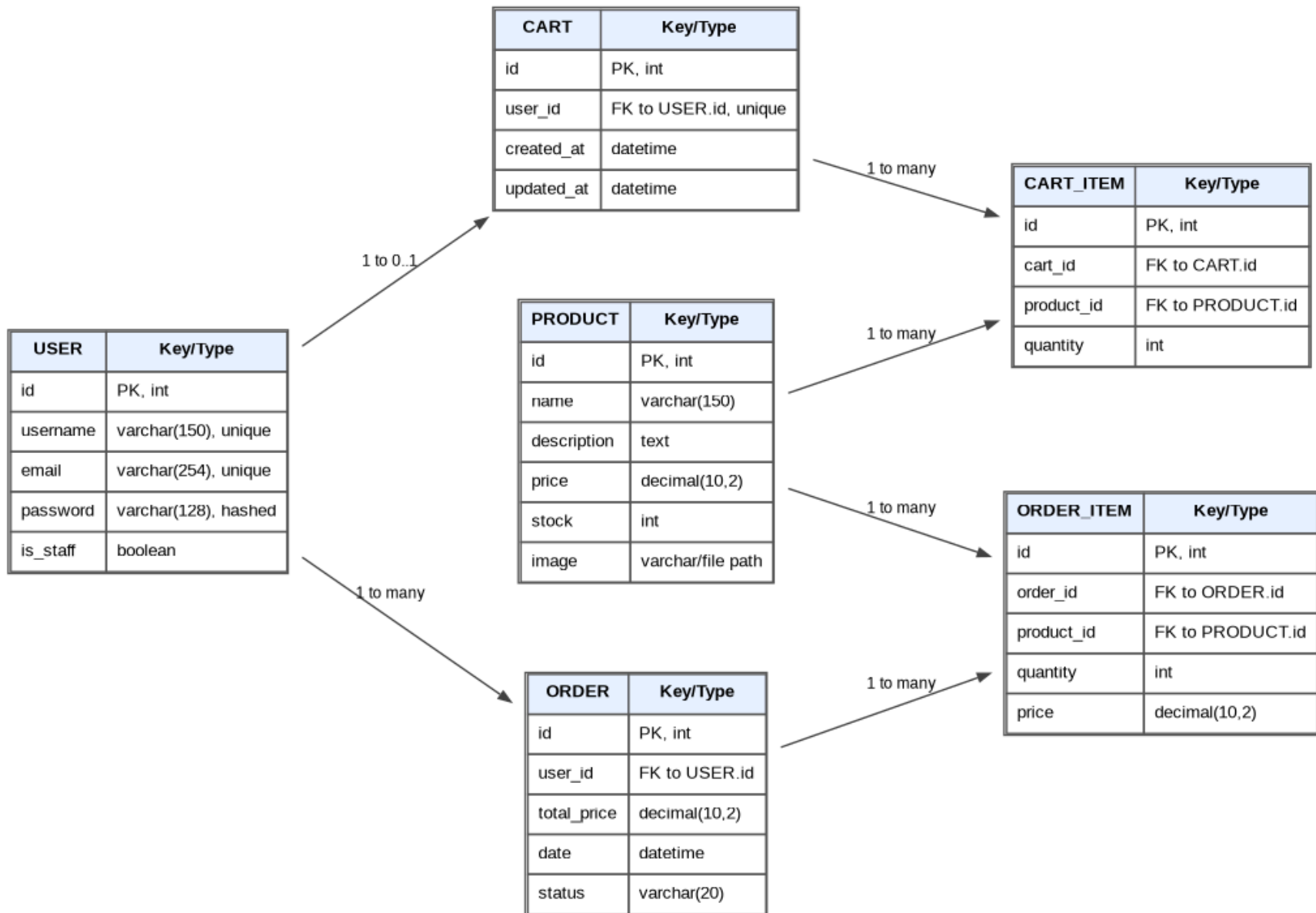
Figure 3: Logical Database Schema / ERD for the E-Commerce Web Application
