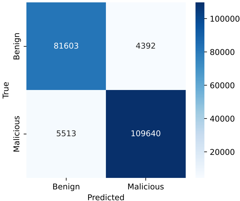
Hybrid Confusion Matrix
