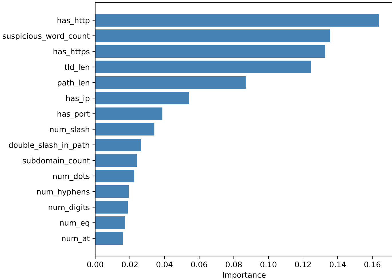
Top URL Features (XGBoost)
