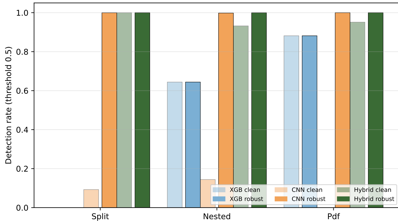
(b) Adversarial Detection: Clean vs Robust ( n = 50,000 / variant)
