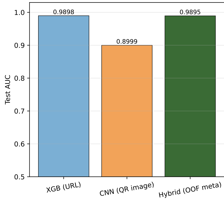
(a) Model Comparison (clean test, n = 40,230 )
