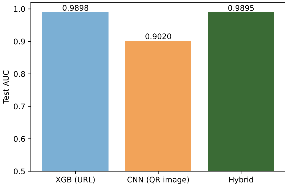
Model Comparison
