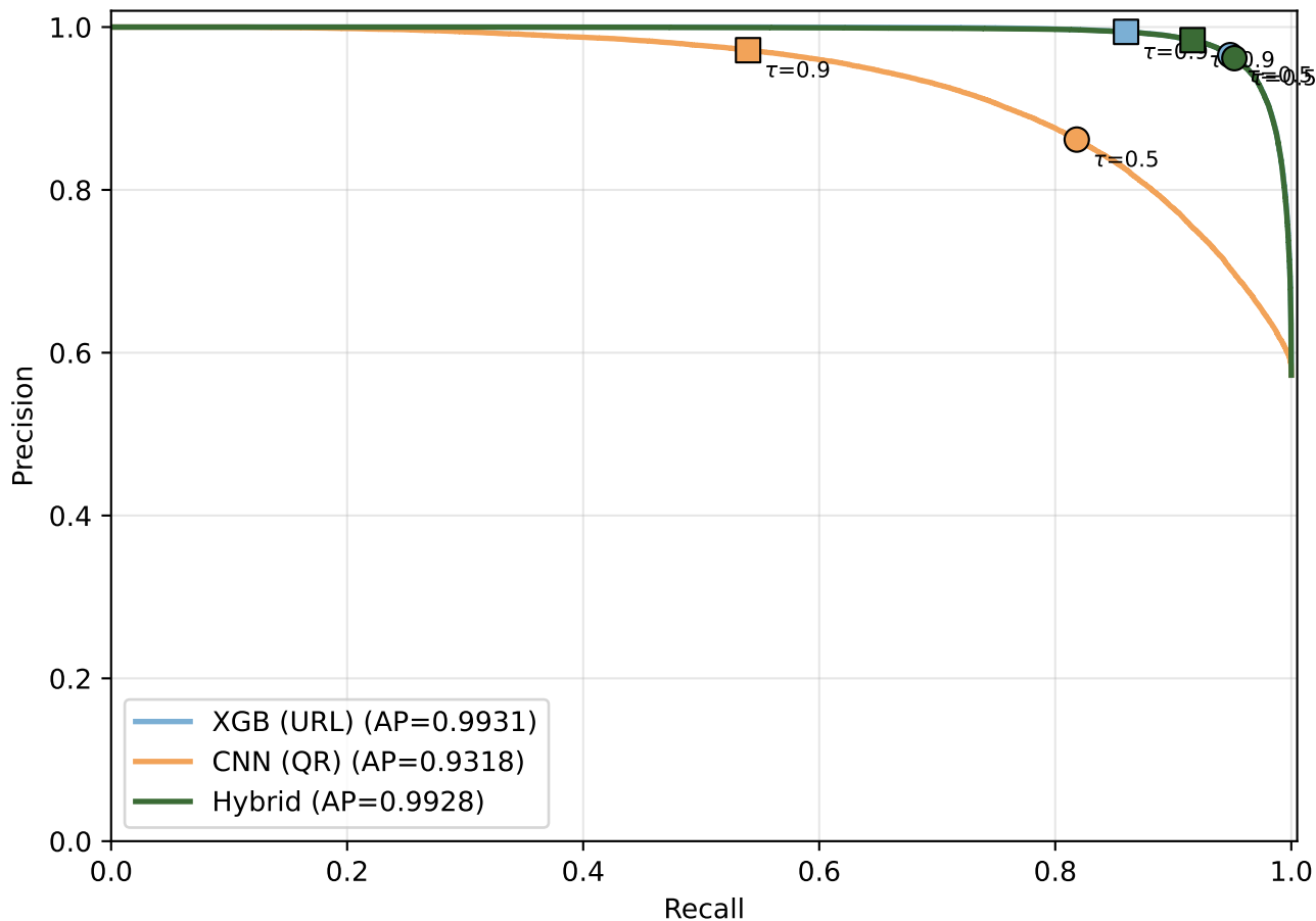
Precision-Recall curves with \tau = 0.5 (•) and \tau = 0.9 (■)
