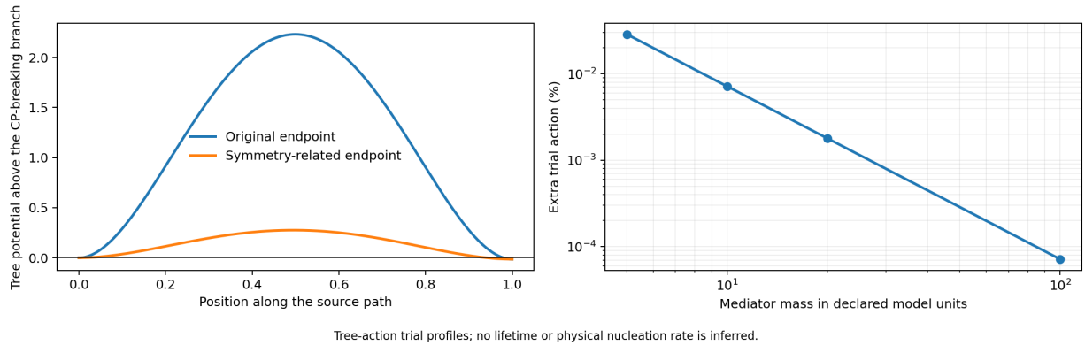
Published fluxor action: trial decay paths and mediator kinetic cost
