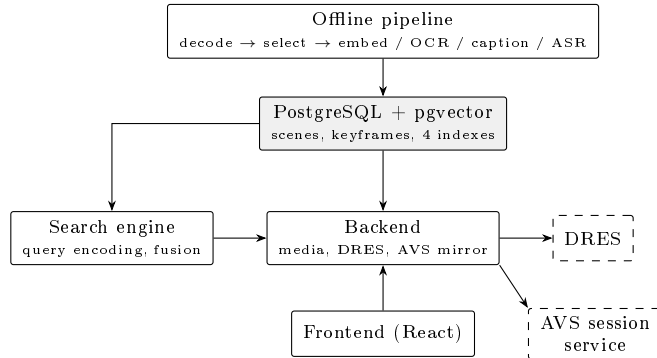
Fig. 1. CLIMB architecture. The offline pipeline writes scenes, keyframes and the four indexes into PostgreSQL before the competition. at query time both the search engine and the backend read from it, the former for ranking, the latter for the scene and keyframe metadata the interface renders. Every component shown runs locally on each operator’s machine, with the exception of the two external services: DRES, and the AVS session service, which is deployed once.
