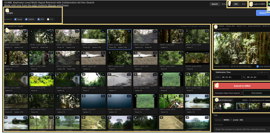
Fig. 2. The CLIMB interface: (a) query bar and source filters, (b) the scene result grid, (c) detail panel with player, (d) submission, and search refinement buttons, (e) keyframe filmstrip, (f) AVS session tab, (g) DRES connection controls and (h) health status overview.
