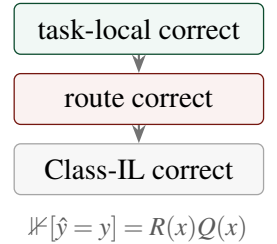
Figure 2: Class-IL needs both events. A prediction is globally correct only when the true task block wins and the correct class wins inside that block.
