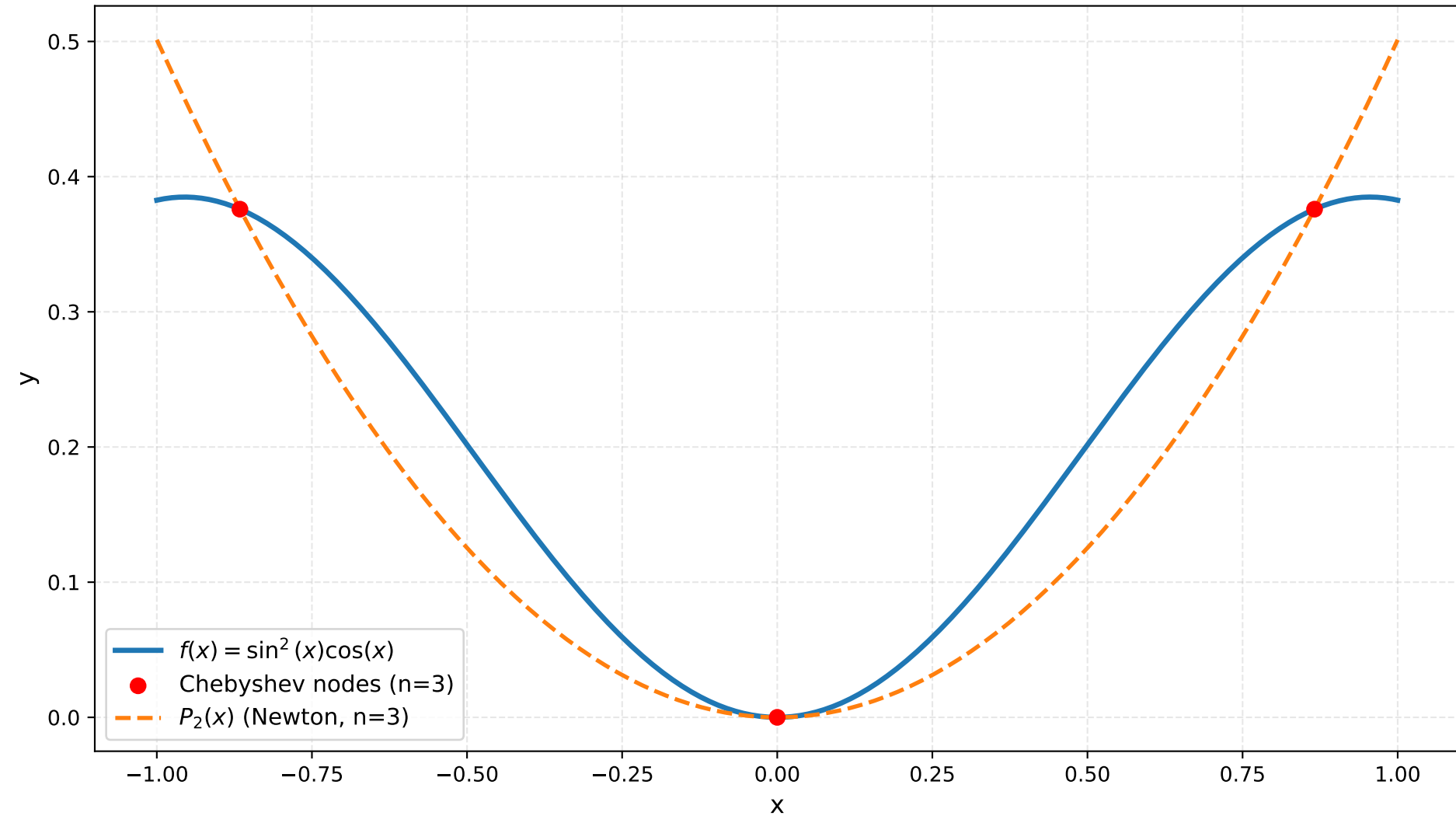
Chebyshev Interpolation on [-1,1] ( n=3 )
