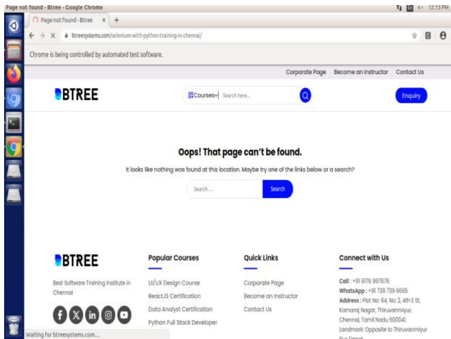
Figure 2. Result.Html
