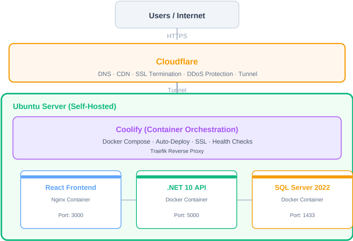
Figure 2: Production deployment — Cloudflare → Coolify → Docker containers
