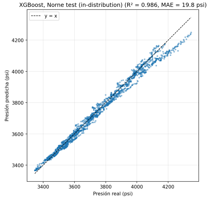
Figura 17: XGBoost, test in-distribution sobre Norne: parity plot global.
