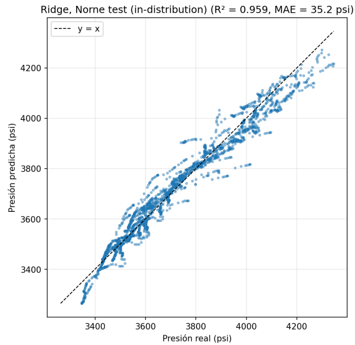
Figura 9: Baseline Ridge, test in-distribution sobre Norne: parity plot global.
