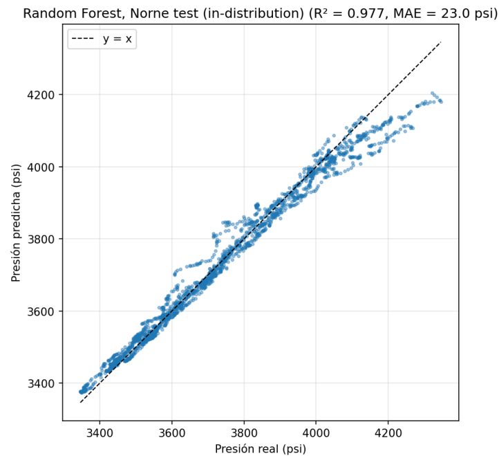
Figura 13: Random Forest, test in-distribution sobre Norne: parity plot global.
