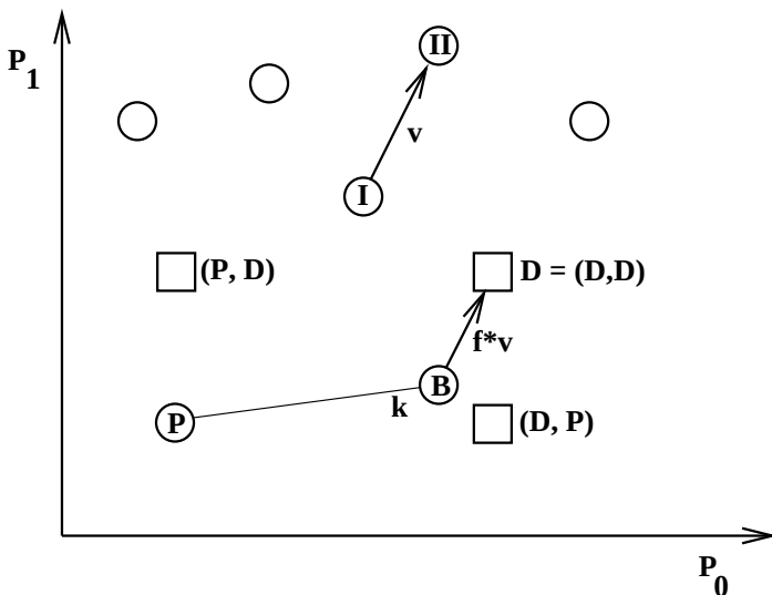
Figure 2.2: Schematic diagram of the differential evolution algorithm.
