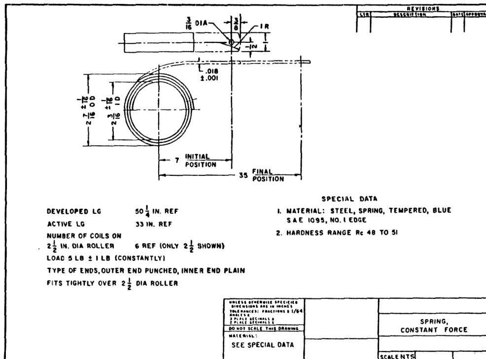
FIGURE 29. Typical detail drawing of constant force spring
