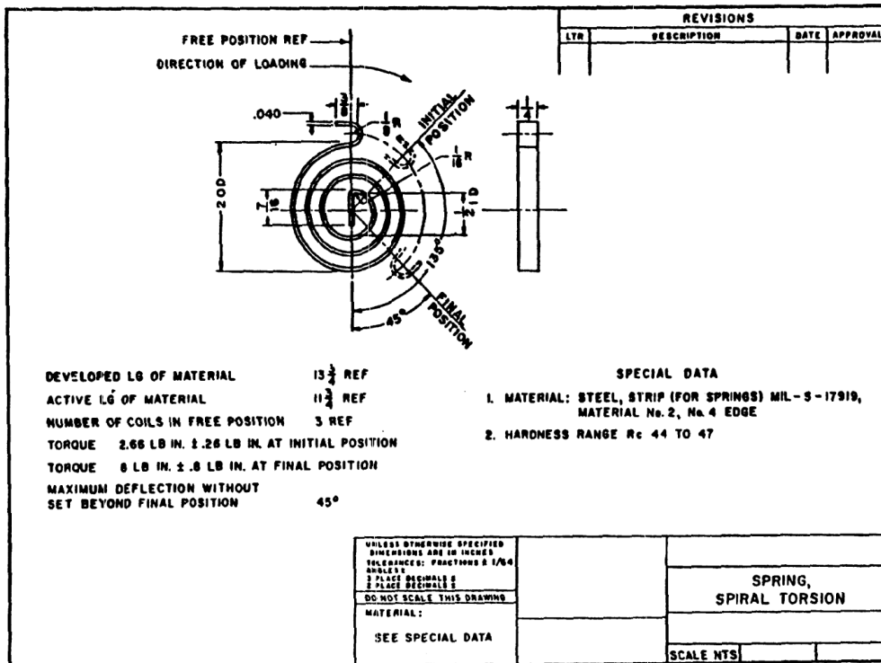
FIGURE 23. Typical detail drawing of spiral torsion spring
