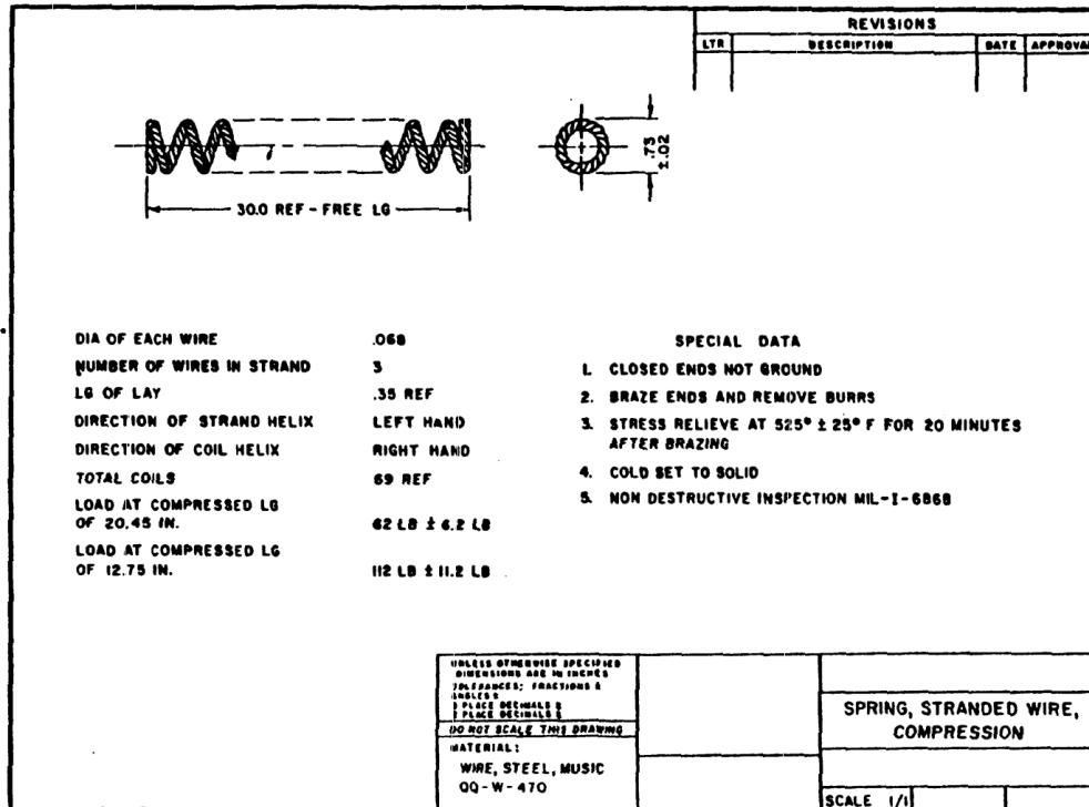
FIGURE 20. Typical detail drawing of stranded wire compression spring
