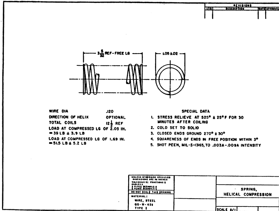
FIGURE 19. Typical detail drawing of compression spring
