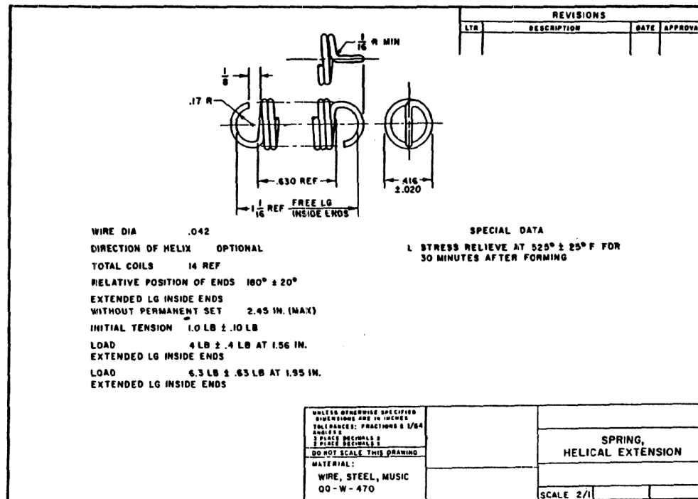
FIGURE 21. Typical detail drawing of extension spring
