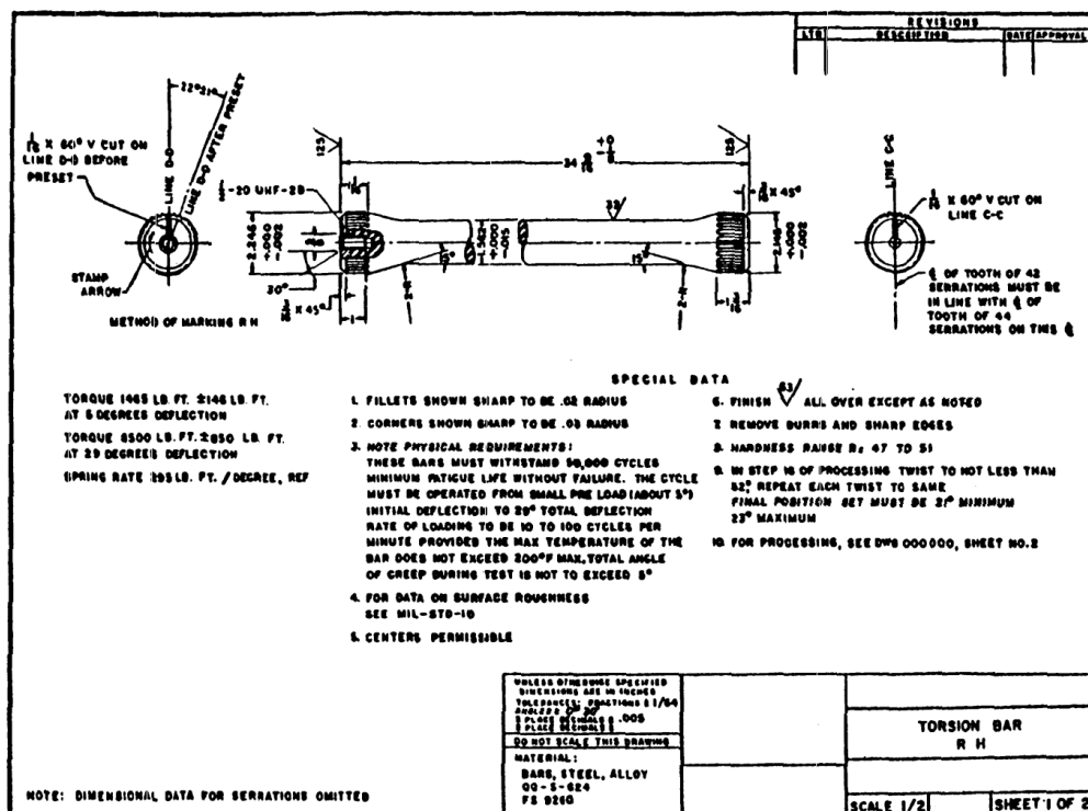
FIGURE 24. Typical detail drawing of torsion bar spring
