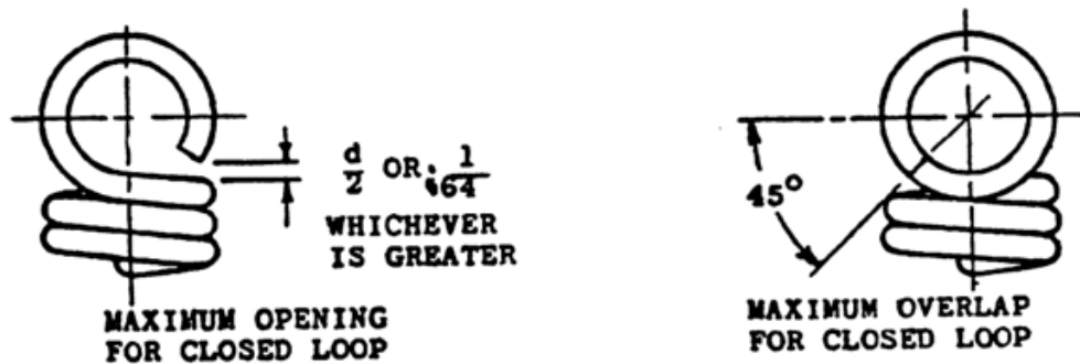
Figure 38: Maximum Deviations Allowed on Ends of Extension Springs
