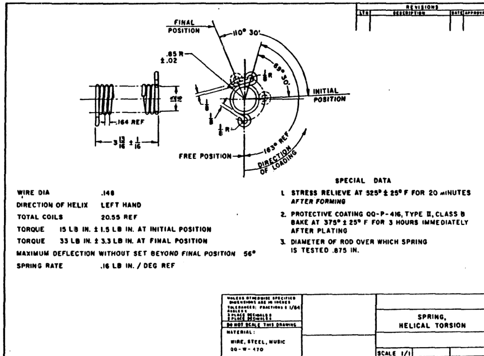
FIGURE 22. Typical detail drawing of helical torsion spring
