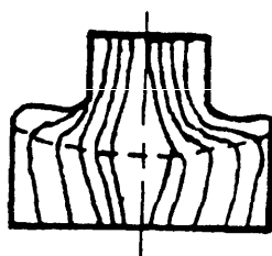
FIGURE 4. Head structure and grain flow.
