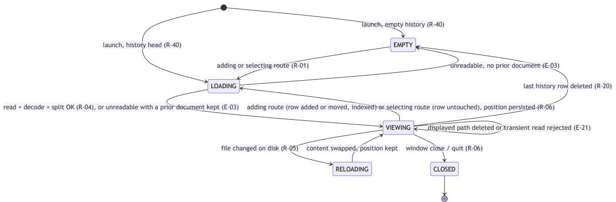
Figure 3.1 — document lifecycle per R-01, R-04..R-06, R-20, R-40, E-03, E-21. The table is normative; the diagram is illustrative.
