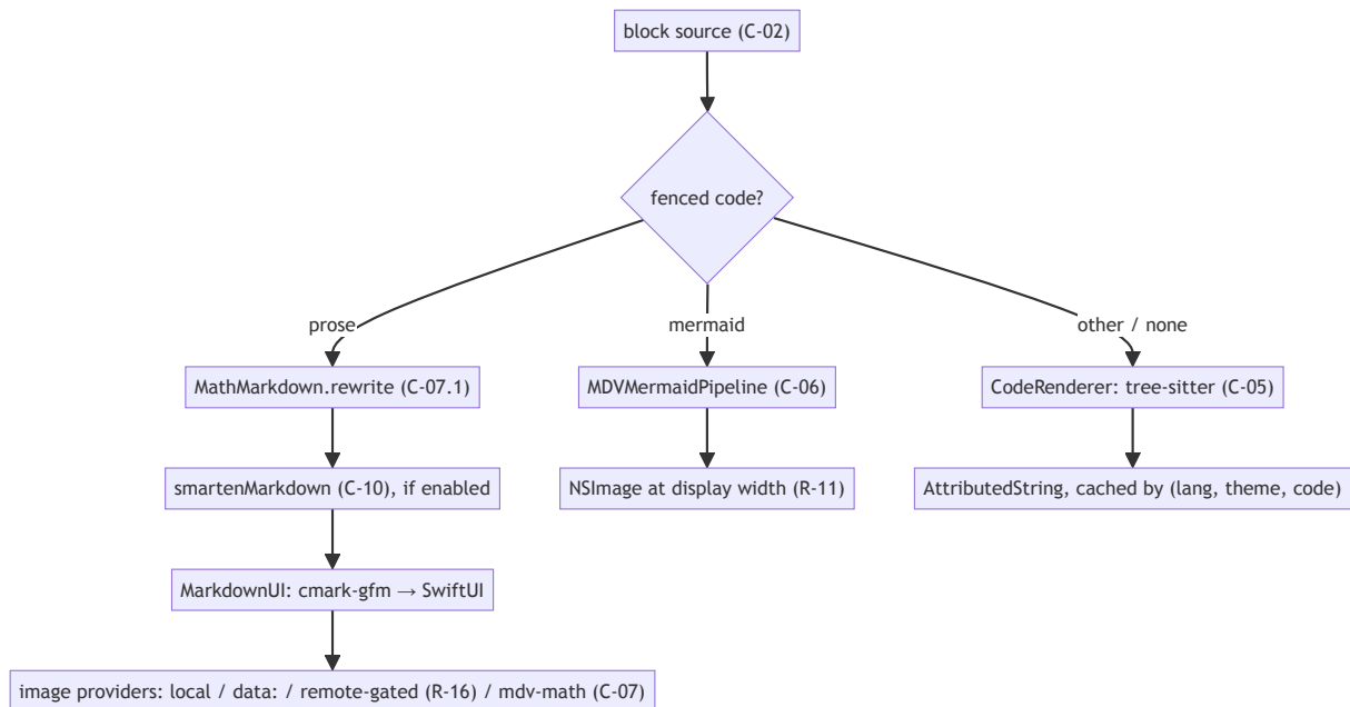
Figure 3.2 — per-block render path per R-07..R-17 . Each edge corresponds to a §4 contract; the diagram is illustrative.
