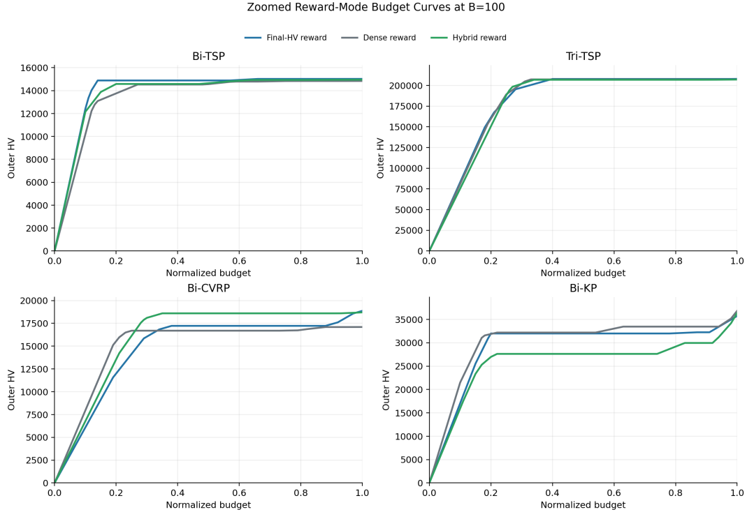
Figure 5.5: Zoomed BMAB-style budget curves at B = 100 , excluding MPaGE-orig to make differences among Final-HV reward, Dense reward, and Hybrid reward more visible.
