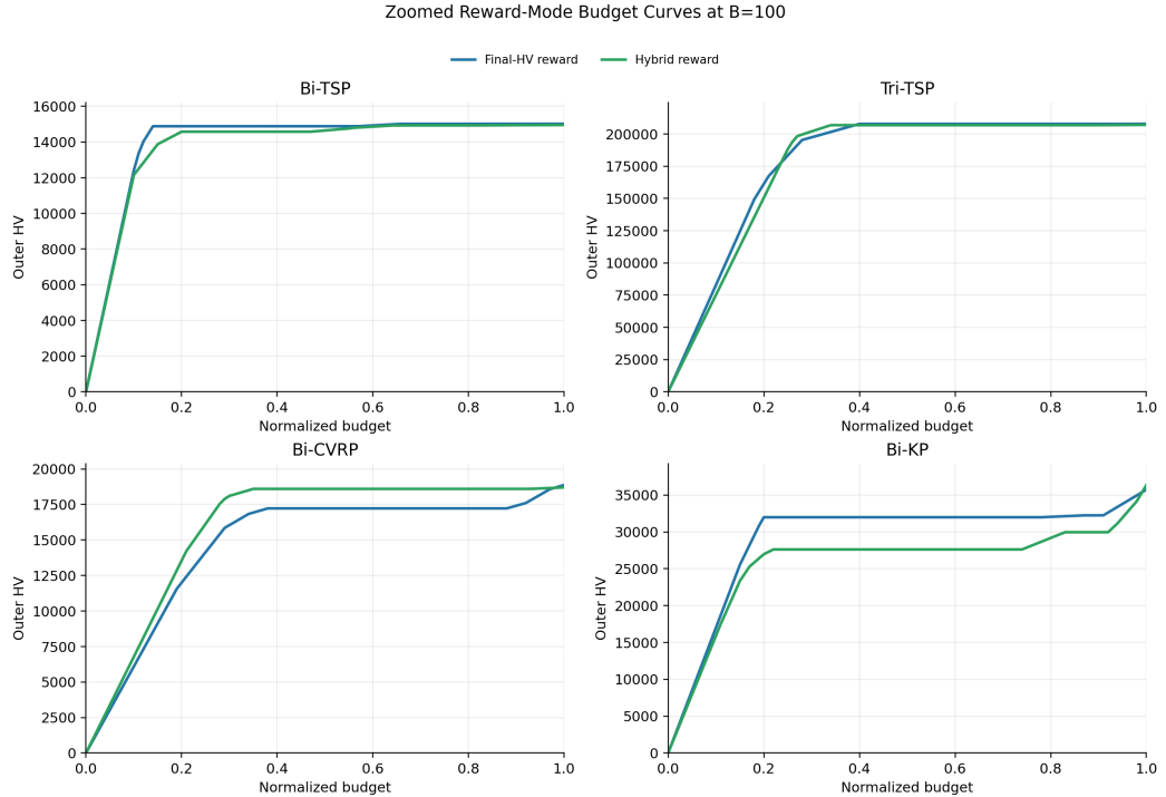
Figure 5.5: Zoomed reward-variant budget curves at B = 100 , excluding MPaGE-orig to make differences between Final-HV reward and Hybrid reward more visible.
