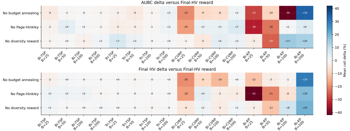
Figure 5.9: Task–budget percentage deltas of the component ablations relative to Final-HV reward. Negative values indicate that the ablation is worse than Final-HV reward in that cell.
