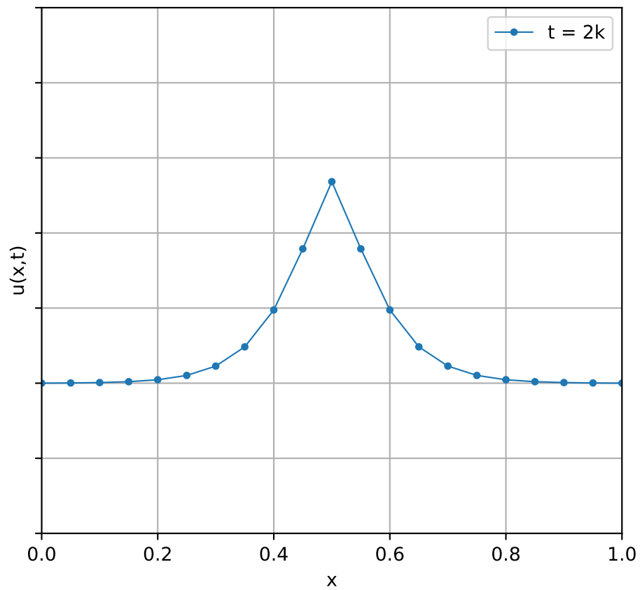
Solution at different times using BTCS method ( r=1.00 )
