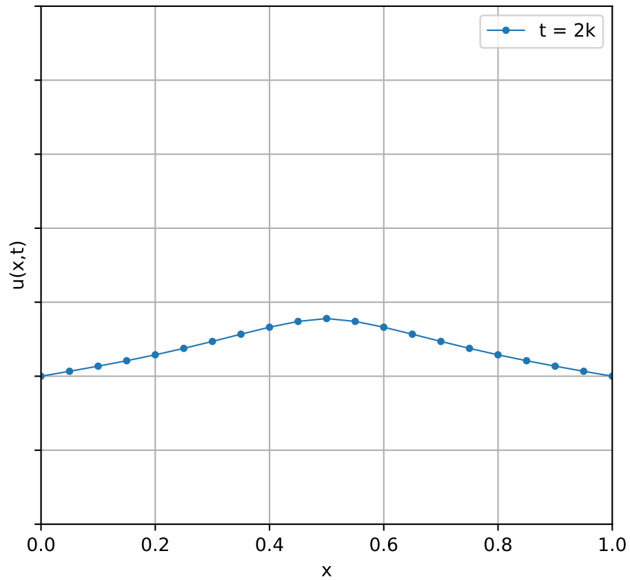
Solution at different times using BTCS method (r=10.00)
