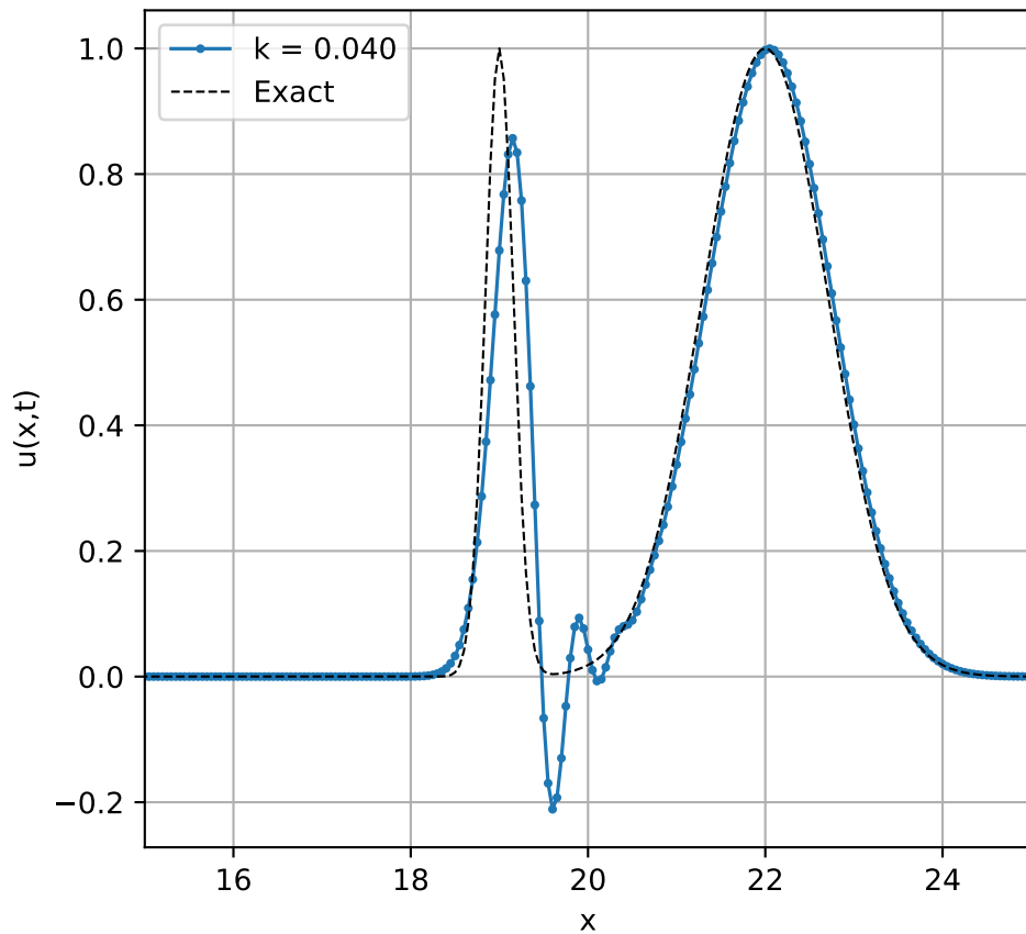
Solution with different k using Beam-Warming method method
