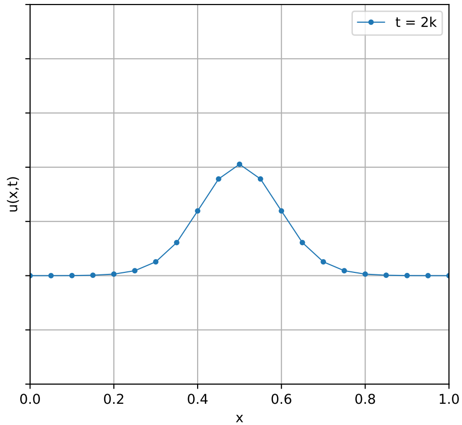
Solution at different times using Collection RK method (r=1.00)
