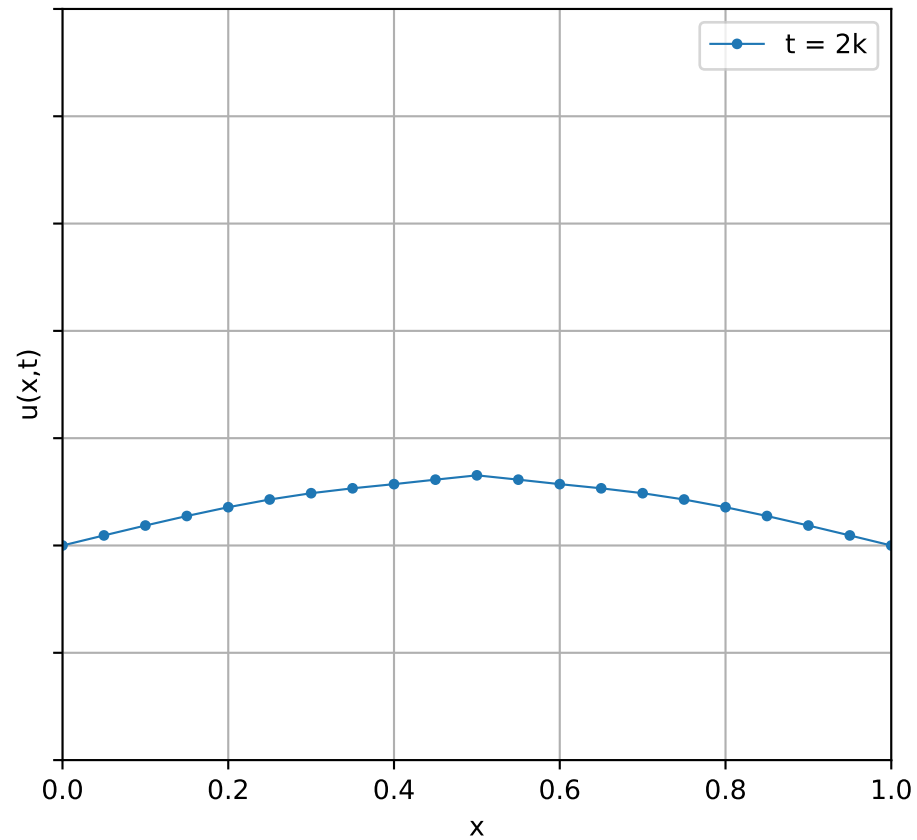
Solution at different times using Collection RK method (r=10.00)
