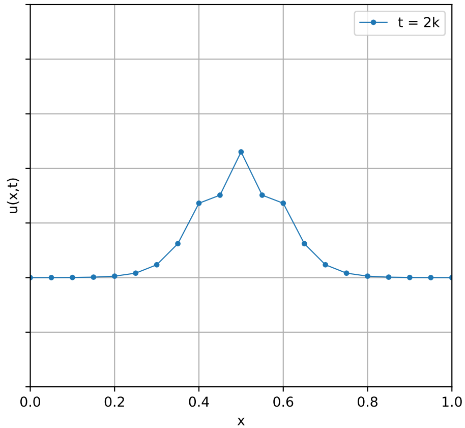
Solution at different times using Crank-Nicolson method ( r=1.00 )
