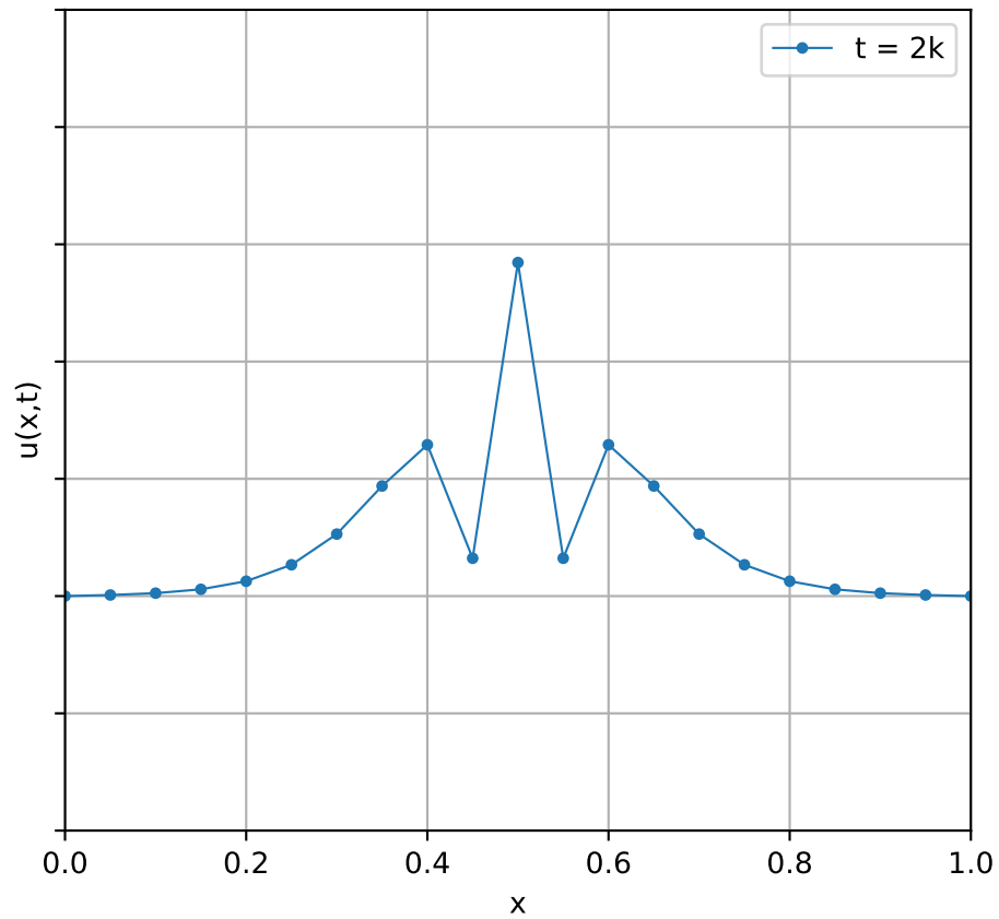
Solution at different times using Crank-Nicolson method ( r=2.00 )
