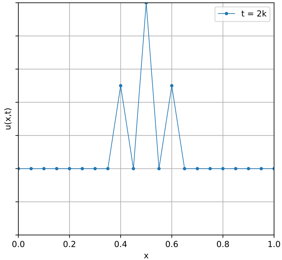
Solution at different times using FTCS method ( r=0.50 )
