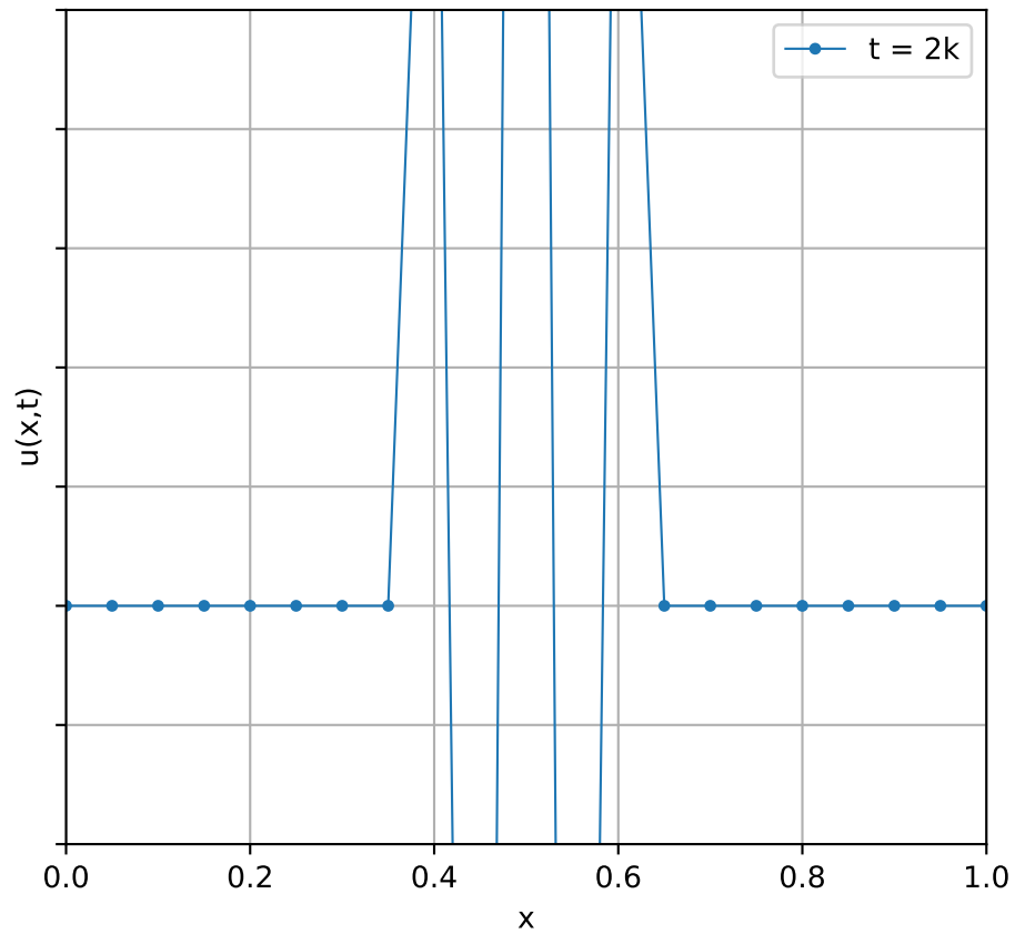
Solution at different times using FTCS method ( r=1.00 )
