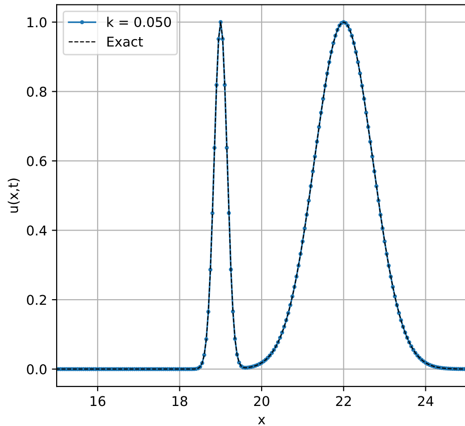
Solution with different k using Lax-Friedrichs method method
