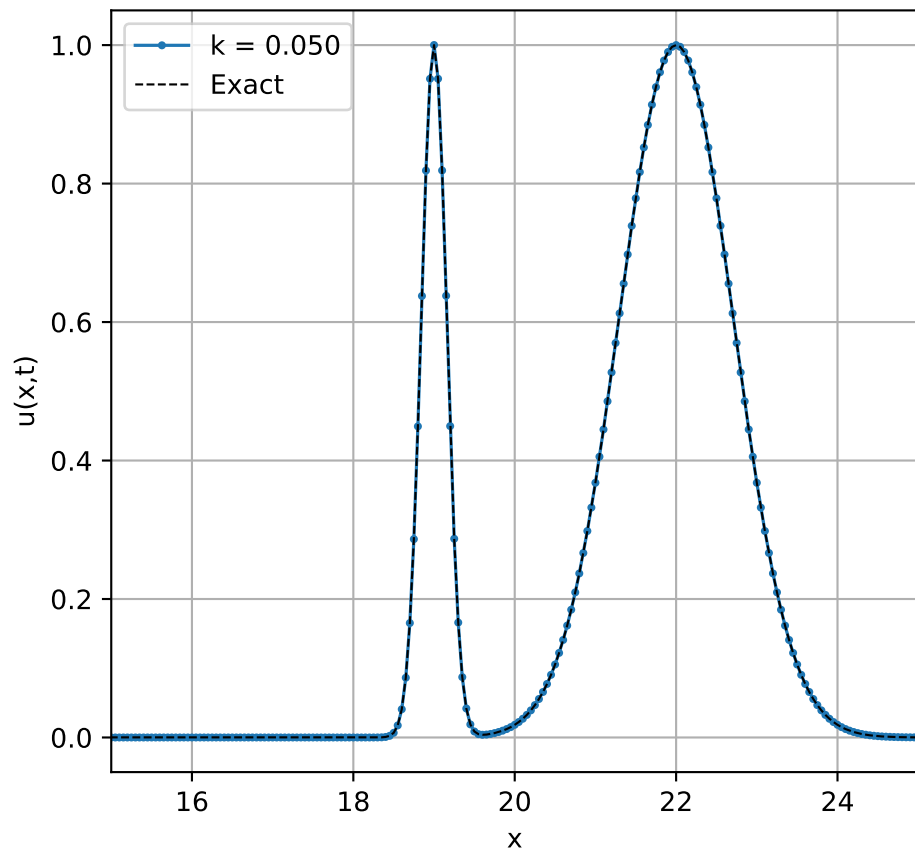
Solution with different k using Lax-Wendroff method method
