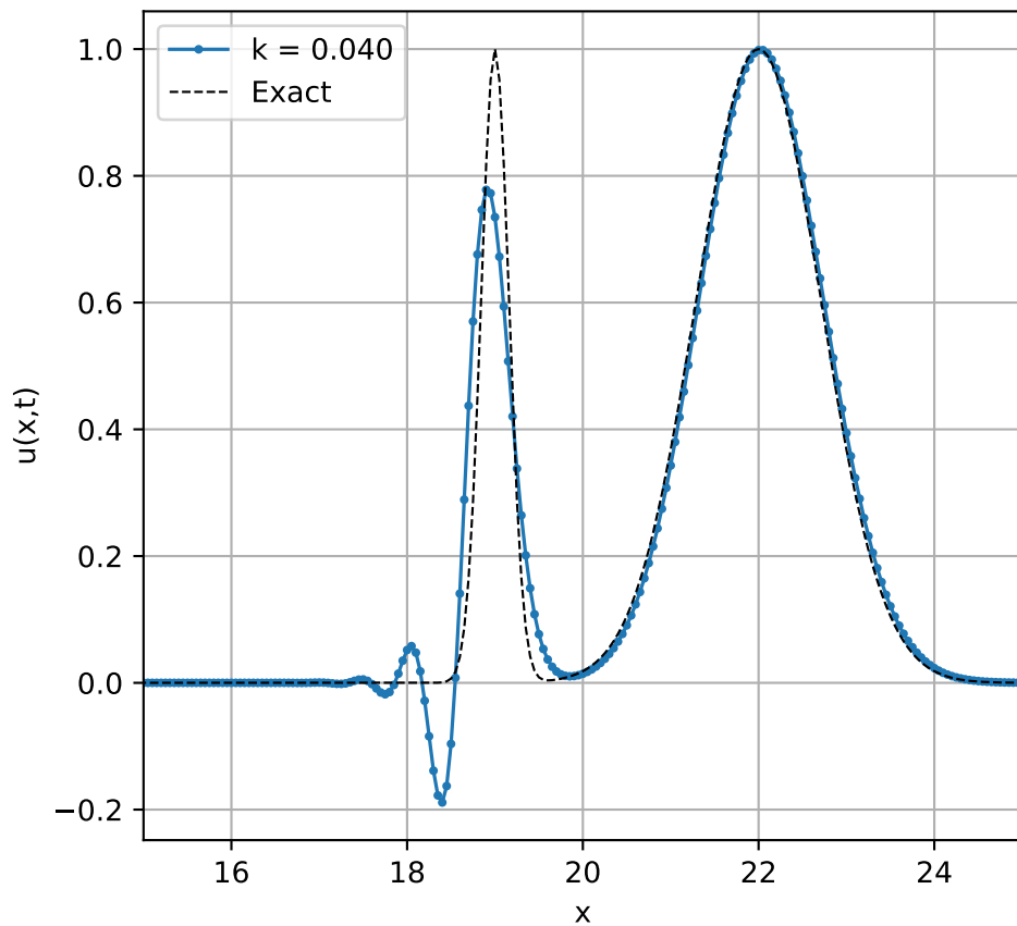
Solution with different k using Lax-Wendroff method method
