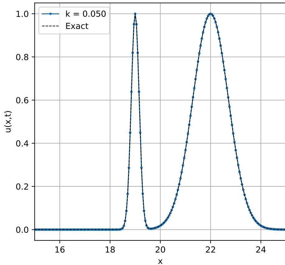
Solution with different k using leapfrog method method
