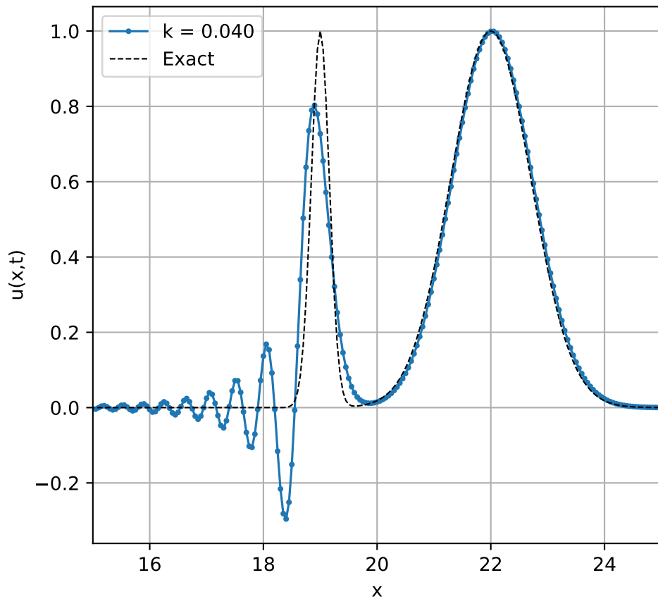
Solution with different k using leapfrog method method
