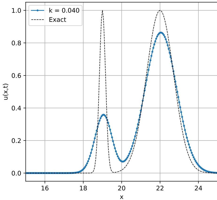
Solution with different k using upwind method method
