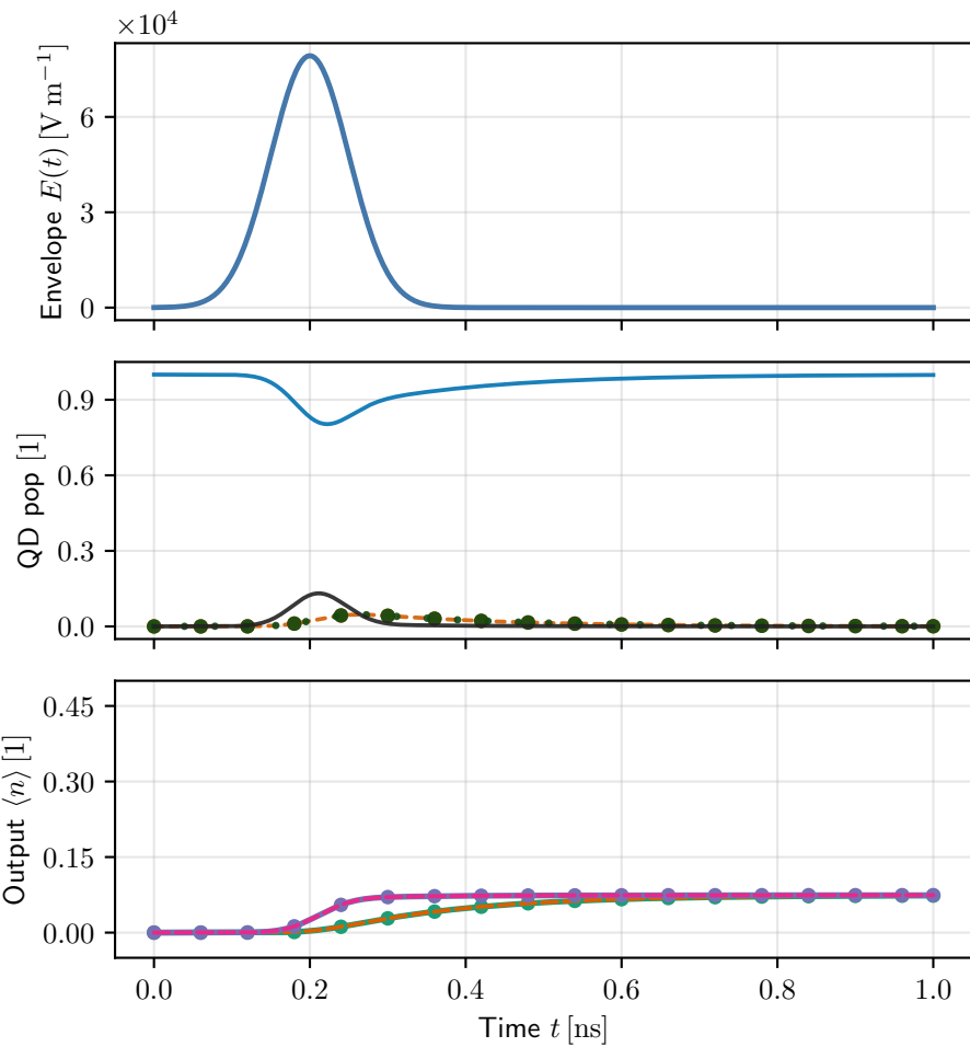
TPE case: tpe_detuned_3GHz
