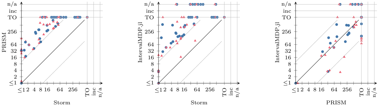
Figure 2: As Figure 1, but with the time each tool reports for model checking only, i.e. without starting the tool and reading and building the model.
