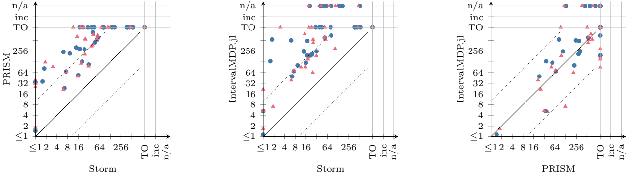
Figure 1: Comparison of Storm, PRISM and IntervalMDP.jl on interval MDPs with interval width \delta . Runtimes are wallclock times of the whole tool call. Top: quantile plot of the runtimes. Bottom: runtimes of pairs of tools. Points marked TO ran out of time or memory, inc disagree with the result most tools agree on, and n/a produced no result or were not applicable, e.g. IntervalMDP.jl on reward benchmarks.
