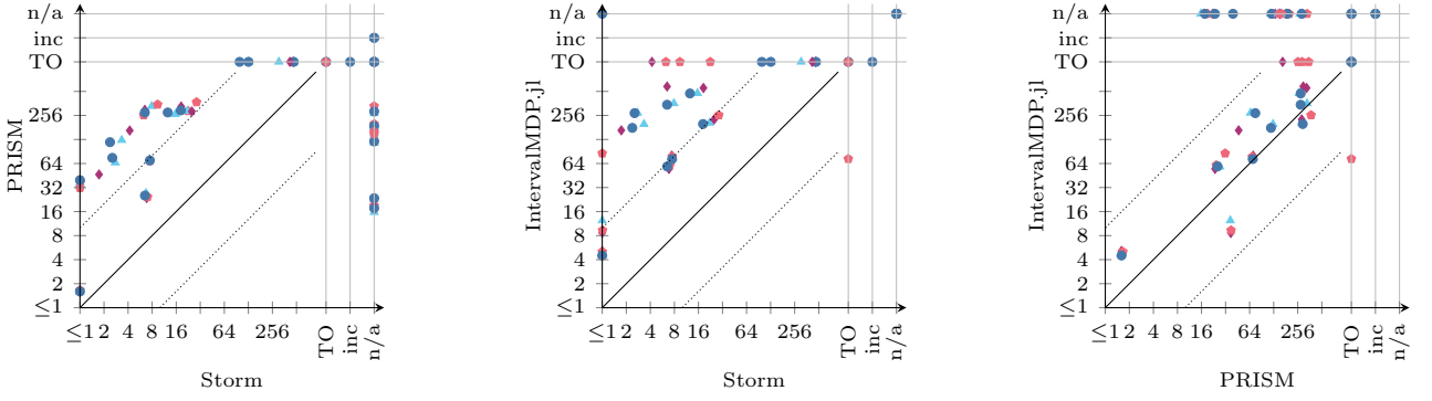
Figure 1: Comparison of Storm, PRISM and IntervalMDP.jl on interval MDPs with interval width \delta . Top: quantile plot of the runtimes. Bottom: runtimes of pairs of tools. Points marked TO ran out of time or memory, inc disagree with the result most tools agree on, and n/a produced no result or were not applicable, e.g. IntervalMDP.jl on reward benchmarks.
