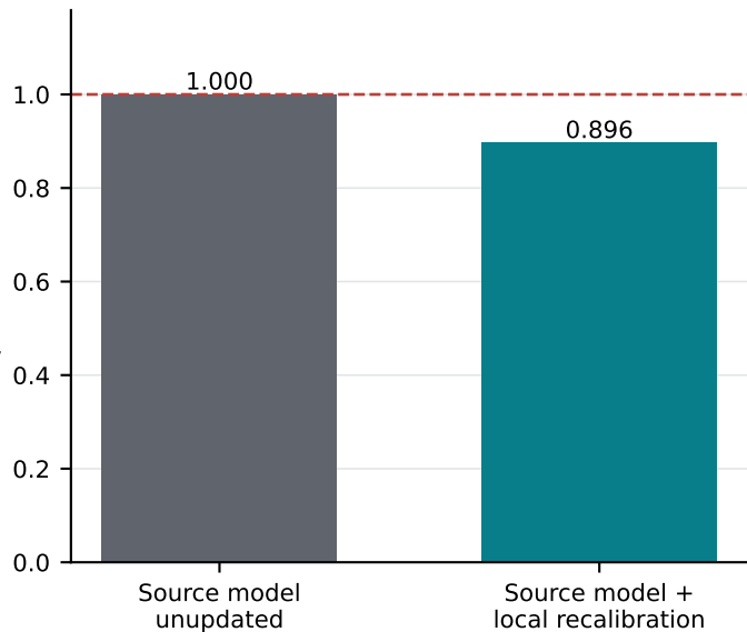
Update beta
