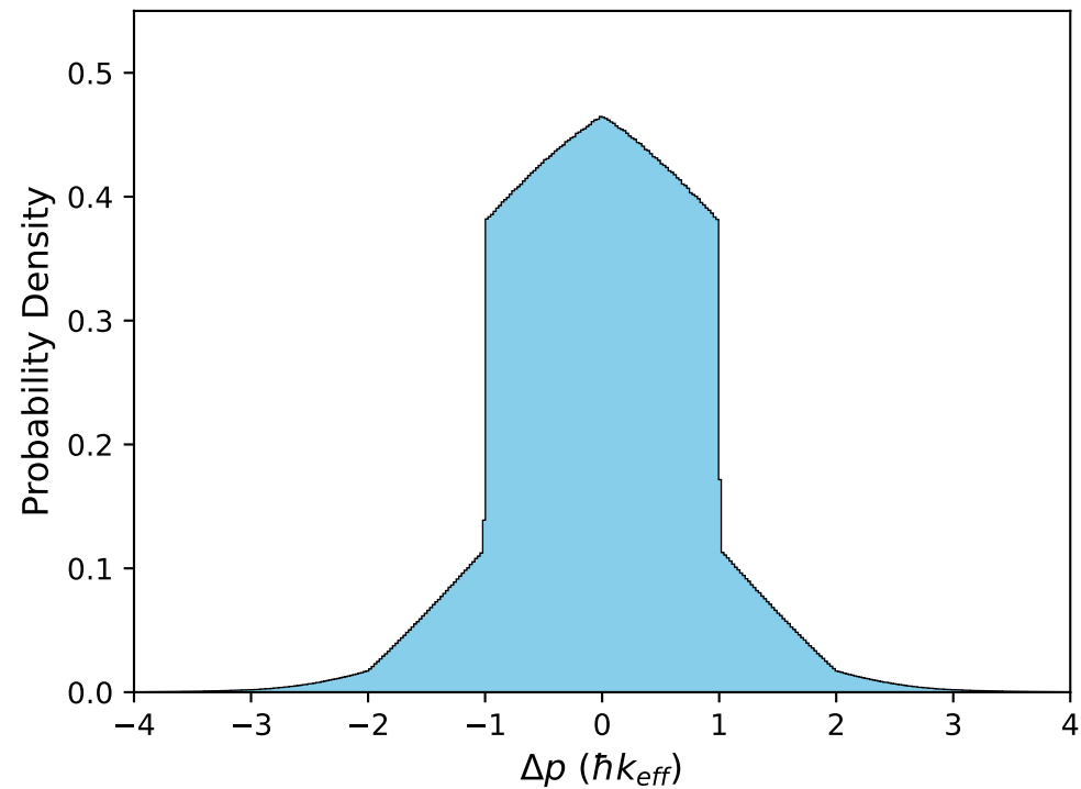
F' = 2 Decay Path, \Delta p_{rms} = 0.795
