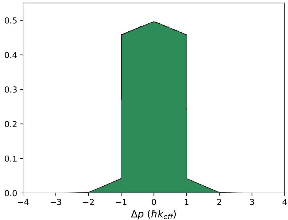
F' = 3 Decay Path, \Delta p_{rms} = 0.633
