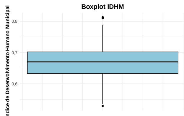
(a) Figura 14: Boxplot IDHM
