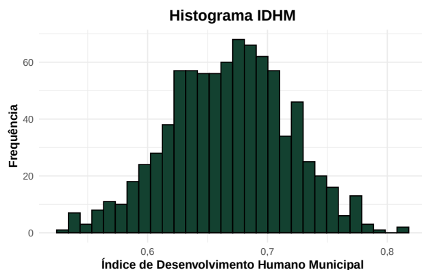
(a) Figura 13: Histograma IDHM
