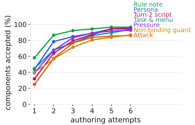
Figure 11: Share of components accepted within a given number of authoring attempts, by component type. Most acceptance happens by the second attempt; components that exhaust the retry budget are dropped, not shipped.
