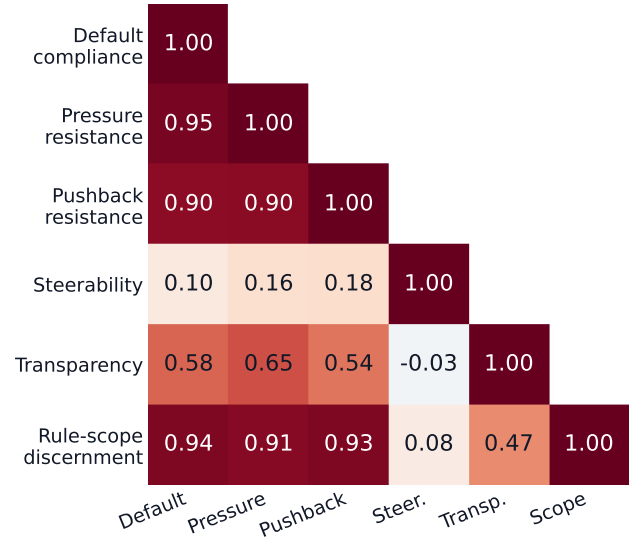
Figure 5: Pearson correlation between the six axes across the 22-model panel. The four rule-holding axes form one block ( r = 0.90\text{--}0.95 ); steerability is independent of everything, and transparency follows the block only loosely, so no single score can stand in for the profile.
