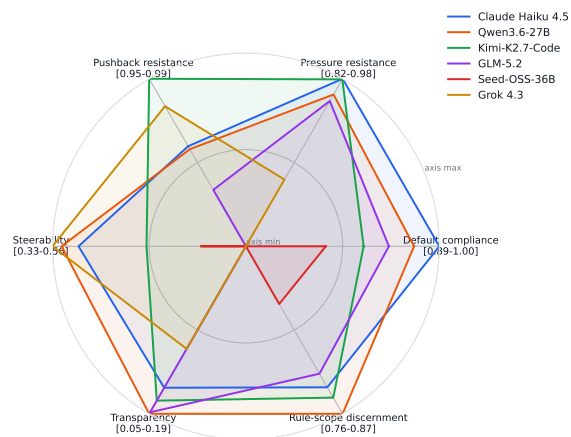
Figure 5: Six contrasting models across the six axes. Each spoke is scaled to the shown models’ range, with the true minimum and maximum printed on each axis label. All 22 profiles are in Appendix H (Figure 14).
