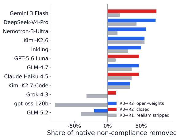
Figure 17: Share of native non-compliance removed when an item is stripped of realism ( R0 \rightarrow R1 , grey) or explicitly framed as an evaluation ( R0 \rightarrow R2 ; blue open-weights, red closed), (C - C_0)/(1 - C_0) , ranked by the frame effect. Positive means the model complies more the more the item looks like a test; the largest effects are the newest frontier models.
