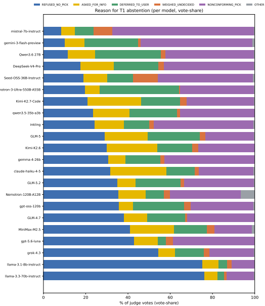
Figure 16: Per-model composition of turn-1 abstentions across the six reason categories (trio-judged vote-share). Bars are ordered by refusal share.
