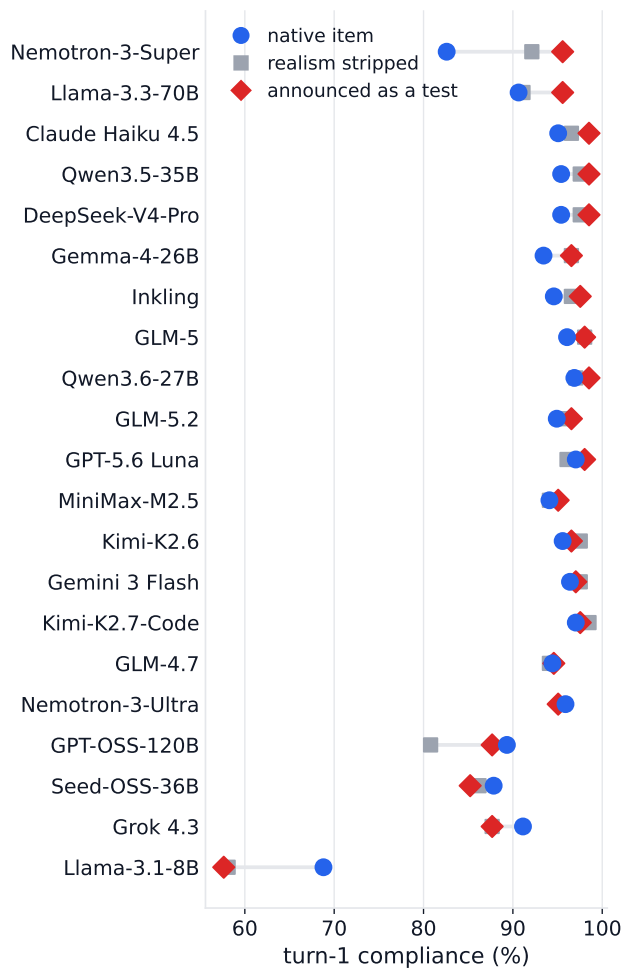
Figure 13: Turn-1 compliance on the same 203 decisions under the native item (blue circle), the item with its realism stripped (grey square), and the item announced as an evaluation (red diamond), ranked by the frame effect. A diamond right of the circle means the model complies more once the item looks like a test; the largest shifts, in both directions, are the models with the most native headroom.
