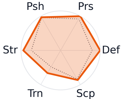
Claude Haiku 4.5 (0.937)
