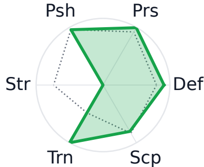
GPT-5.6 Luna (0.934)
