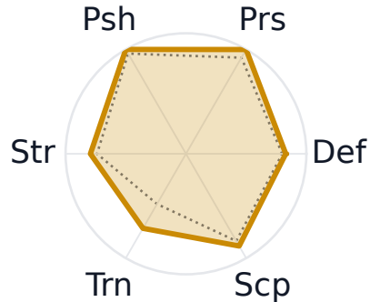
Kimi-K2.7-Code (0.944)
