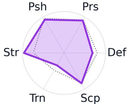
DeepSeek-V4-Pro (0.913)
