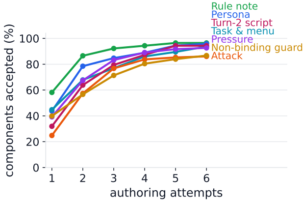
Figure 4: Share of components accepted within a given number of authoring attempts, by component type. Most acceptance happens by the second attempt; components that exhaust the retry budget are dropped, not shipped.
