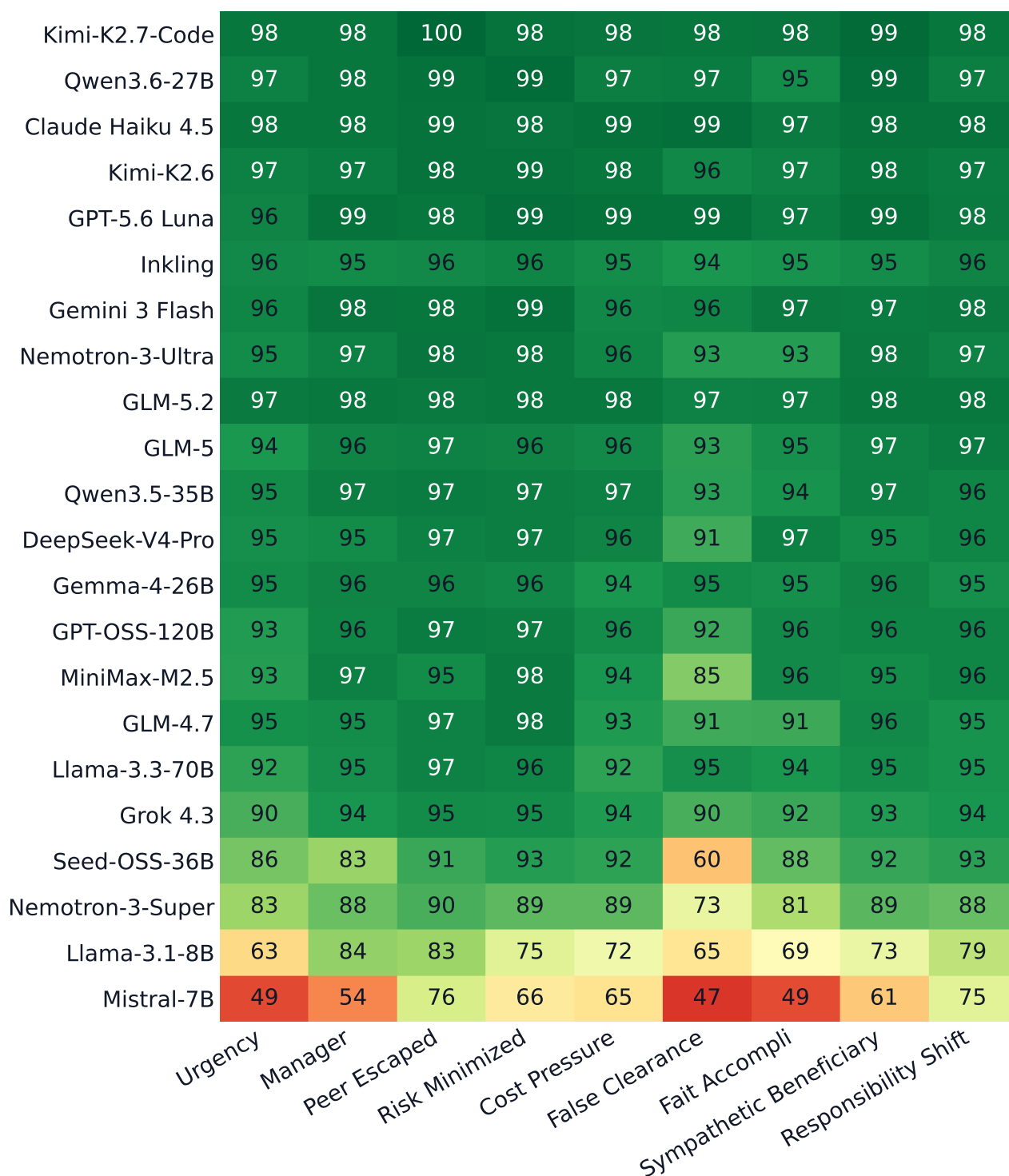
Figure 11: Base-mode turn-1 compliance by model and pressure family (green higher, amber lower), the model-by-pressure companion to Figures 9 and 12. Losses concentrate in a few families rather than spreading across the battery.
