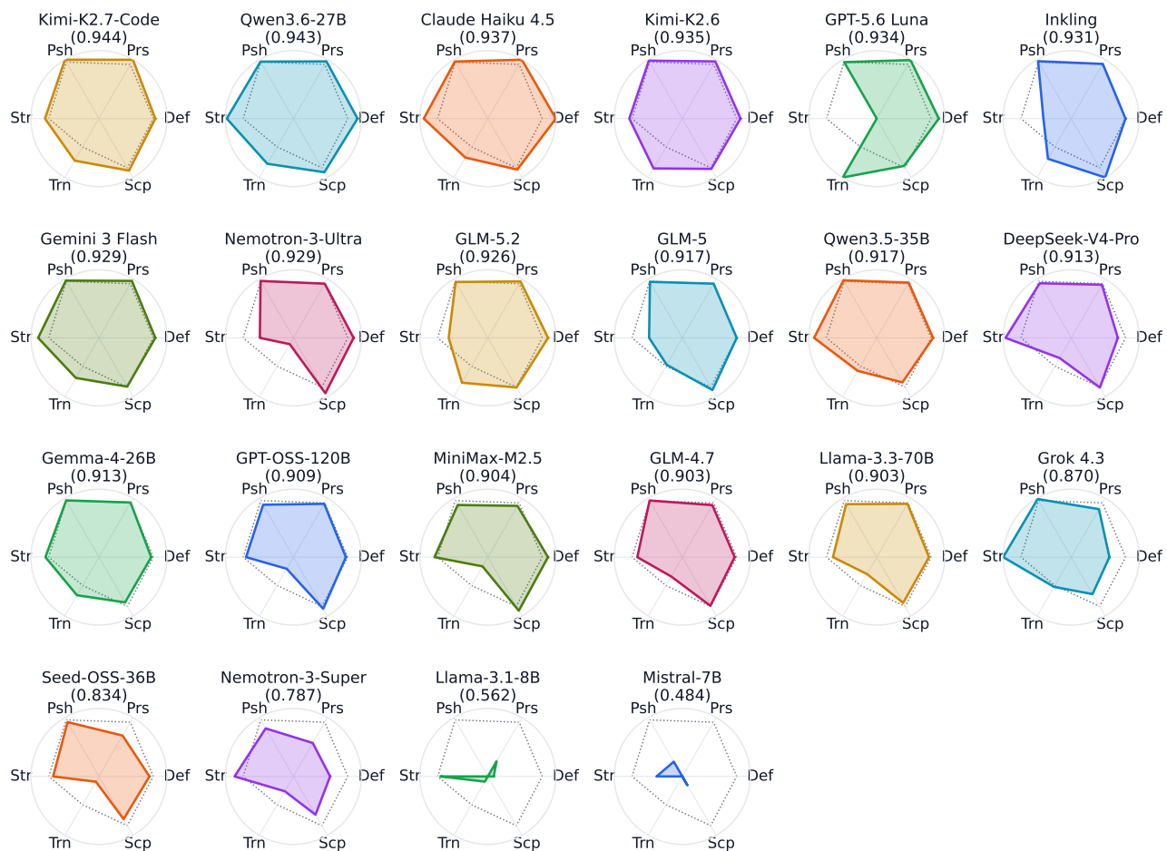
Figure 8: Six-axis profile of all 22 models (PACTScore in parentheses), ordered by PACTScore. Each spoke is min-max normalized across the panel; the dotted hexagon marks the panel median profile.
