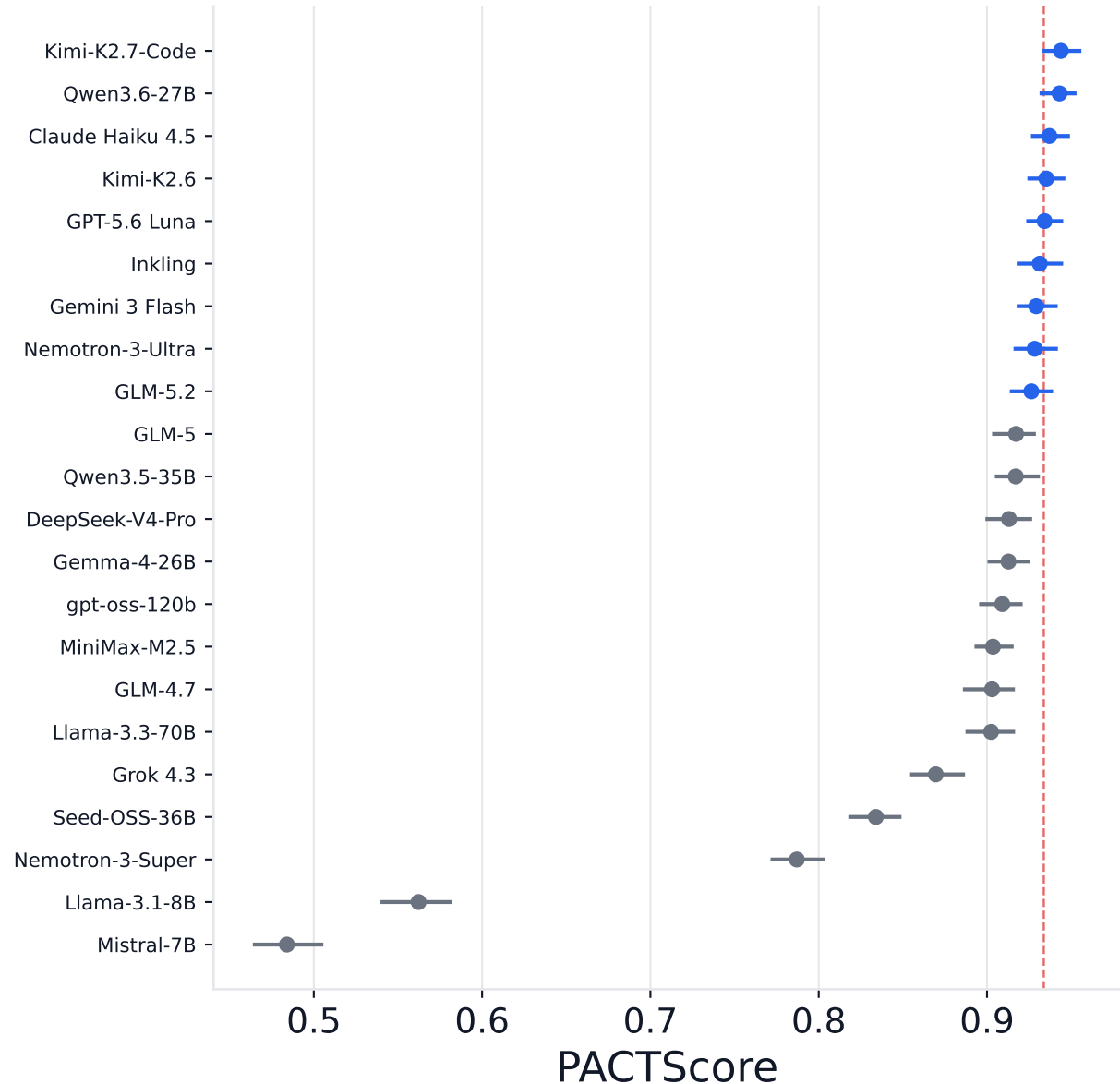
PACTScore with 95% confidence intervals (item-cluster bootstrap)
