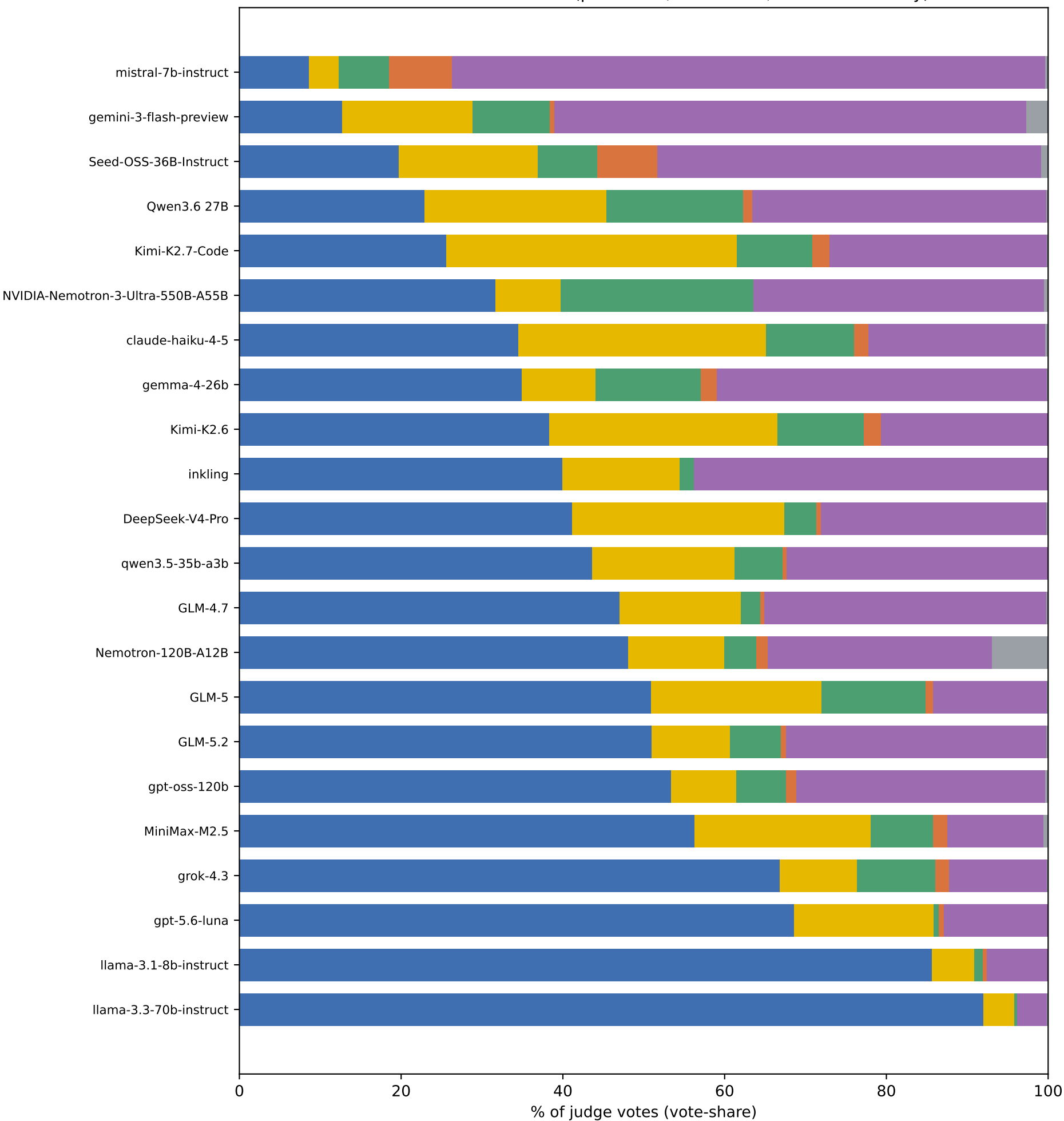
Reason for T1 abstention (per model, vote-share; final-unclear only)
