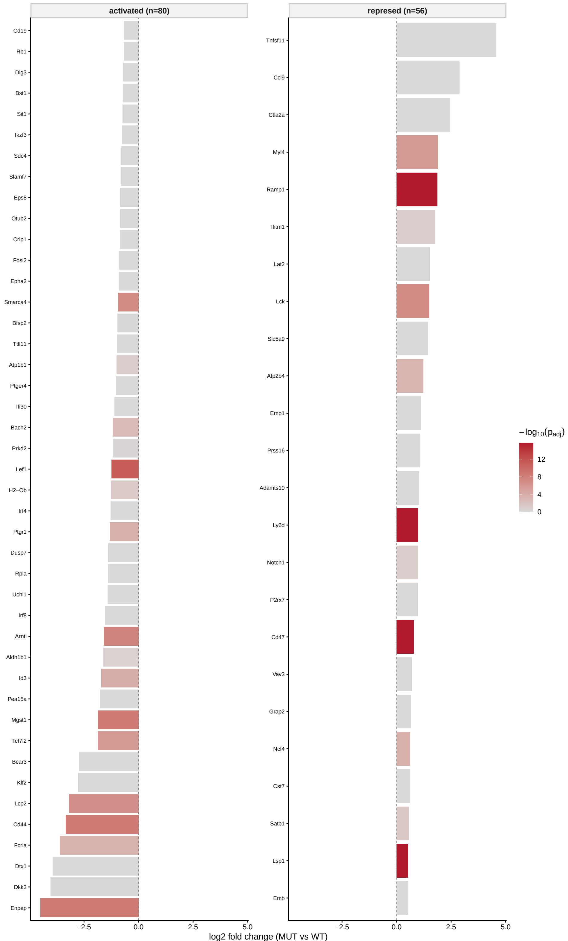
Leading edge genes – ProB (MUT vs WT)
