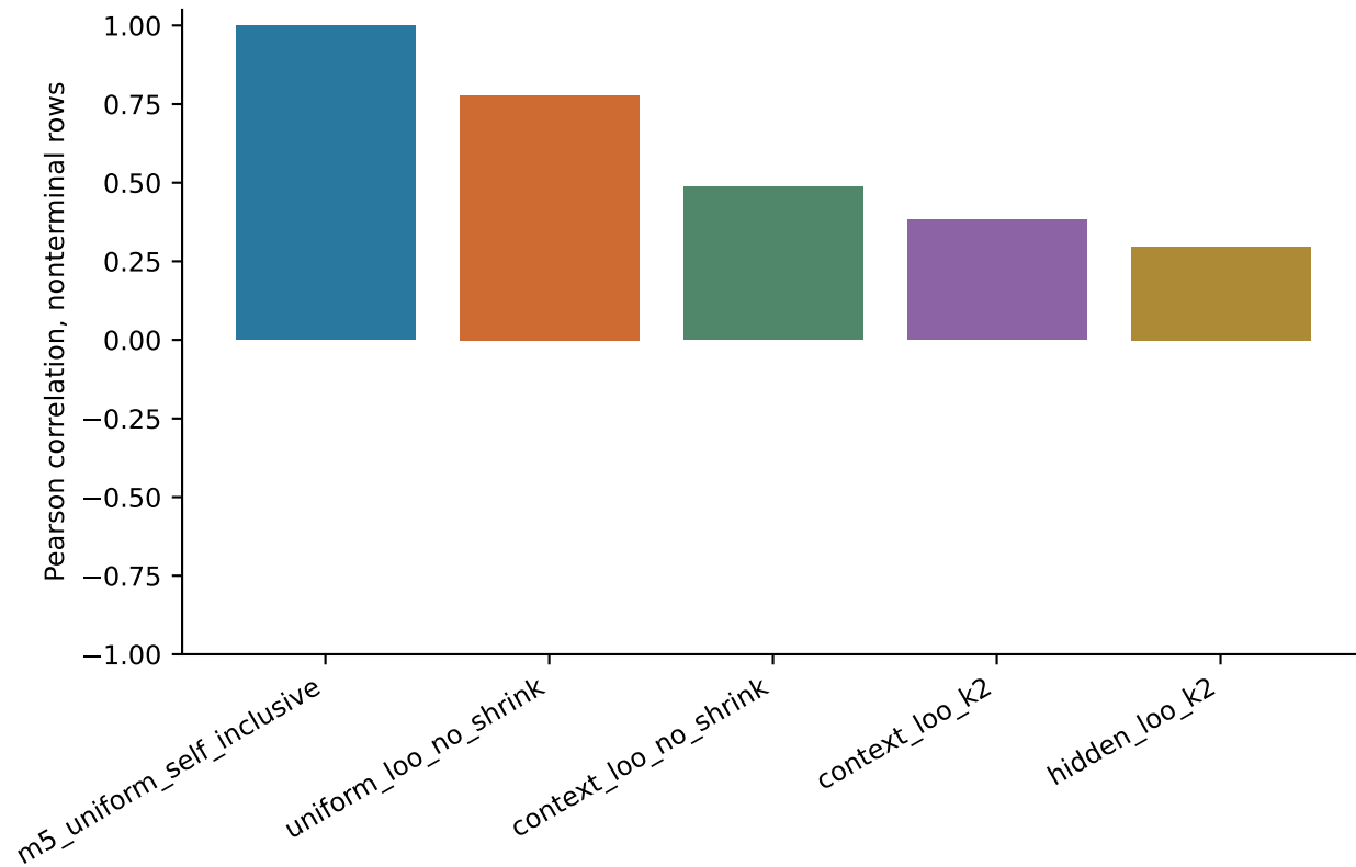
M11: edge readout changes, H1 fixed
