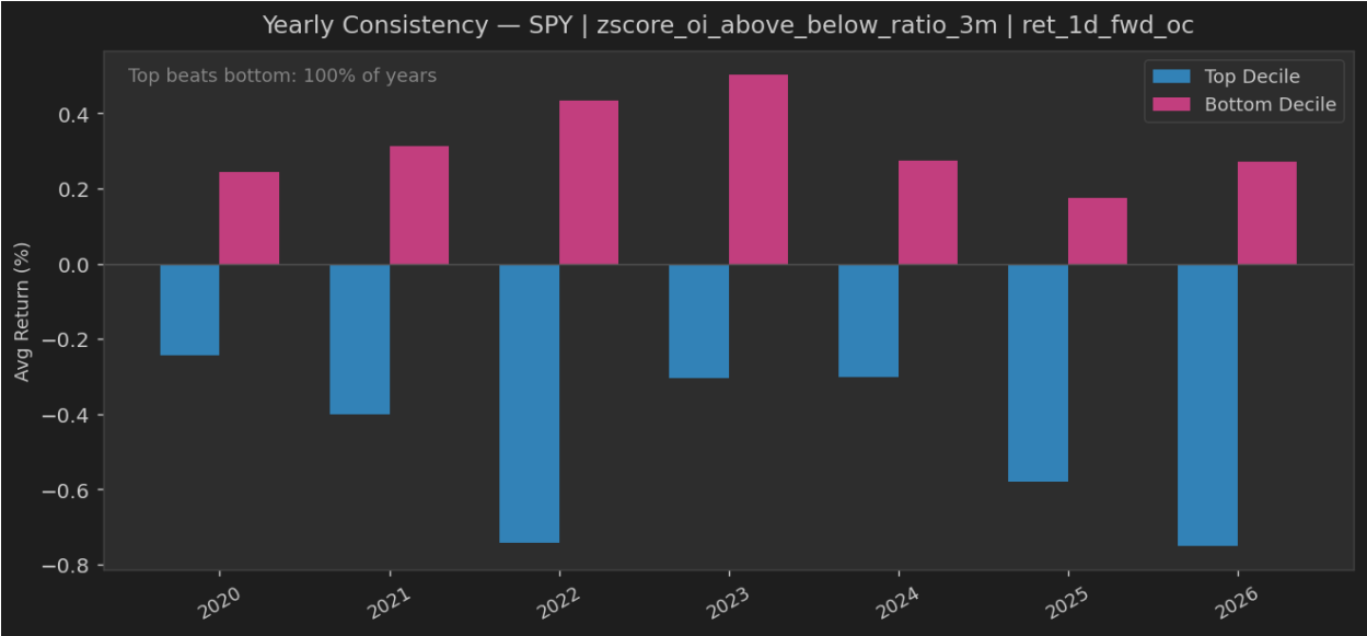
Yearly SPY | zscore_oi_above_below_ratio_3m → ret_1d_fwd_oc
